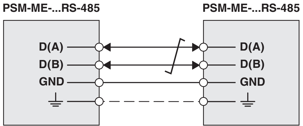
Connection diagram
